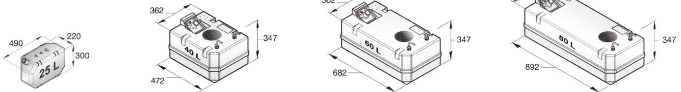
Dimensions: plus or minus 2%. Height dimensions includes connectors.
