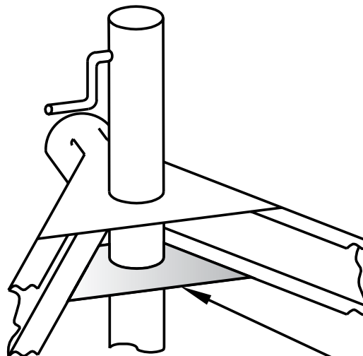
6612 Support Bracket
